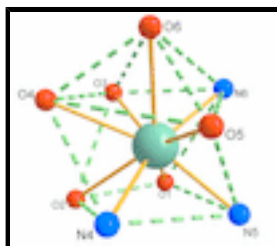
Fig. 2. The coordination environment of the Pr III .
